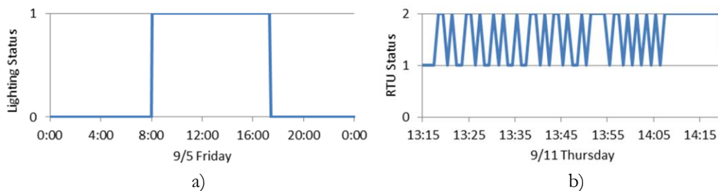
Figure 5. Trends from sensors: (a) Site B, trend from a lighting status sensor (1=lighting on, 0=lighting off) on a weekday during the monitoring period, (b) Site B, example trend from a rooftop unit status sensor (0=off, 1= supply fan only on, and 2= compressors, condenser fans, and supply fan all on) during the monitoring period
