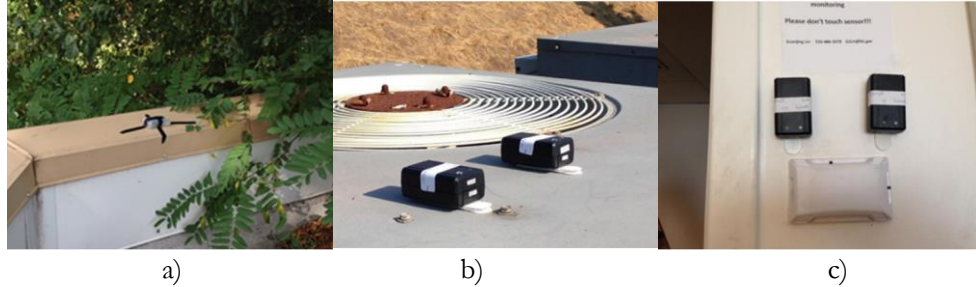
Figure 4. Photos of (a) an outdoor air temperature sensor placed on the north side of the roof, (b) two rooftop unit sensors mounted on top of an RTU, and (c) two indoor air temperature sensors placed near a thermostat.
